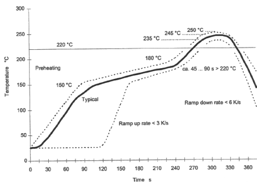
Lead free SnAgCu solders – Infrared Soldering
